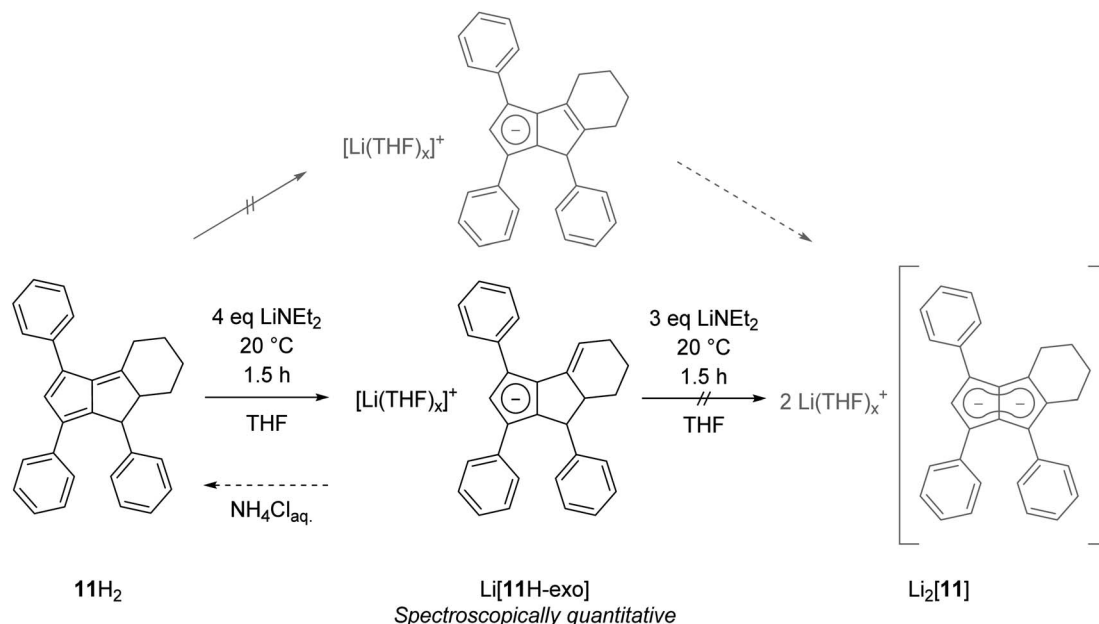
Scheme 6 Exocyclic deprotonation of 11\text{H}_2 to 11\text{H-exo} .
