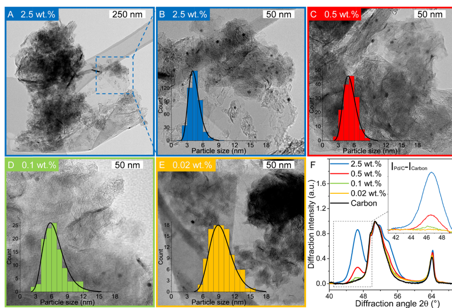
Fig. 2 Catalyst characterisation. (A–E) Transmission Electron Microscopy (TEM) images of Pd/C catalysts with Pd weight loading of (A) 2.5 wt% and high (B) and high magnification, (C) 0.5 wt% (D) 0.1 wt% and (E) 0.02 wt%. Insets shown size histograms of the individually measured diameters from TEM and lognormal fit to the distribution. (F) X-ray diffractogram of the Pd/C catalysts. The inset shows the carbon-subtracted intensity, highlighting the Pd(111) diffraction at 46.6° 2θ.
