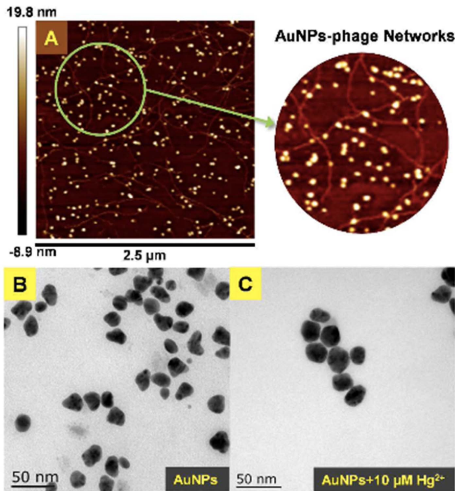
Fig. 12 (A) AFM image and (B and C) TEM images of AuNPs-phage network without and with the addition of Hg(II) (reproduced from ref. 89 with permission from Royal Society of Chemistry, Copyright © 2017).
