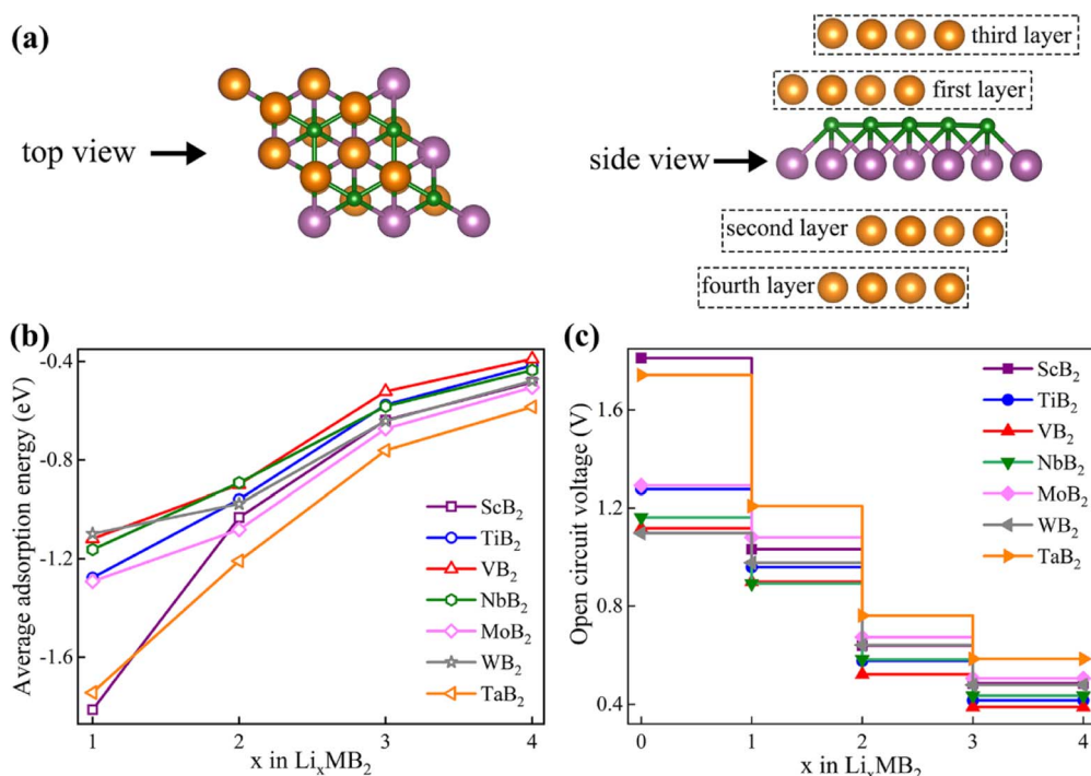
Fig. 5 (a) The structural configuration of four layers of Li atoms adsorbed on the surface of MB 2 ; (b) the change in average adsorption energy and (c) the open circuit voltage of LixMB 2 (M = Sc, Ti, V, Nb, Mo, W and Ta) as a function of Li concentration.
