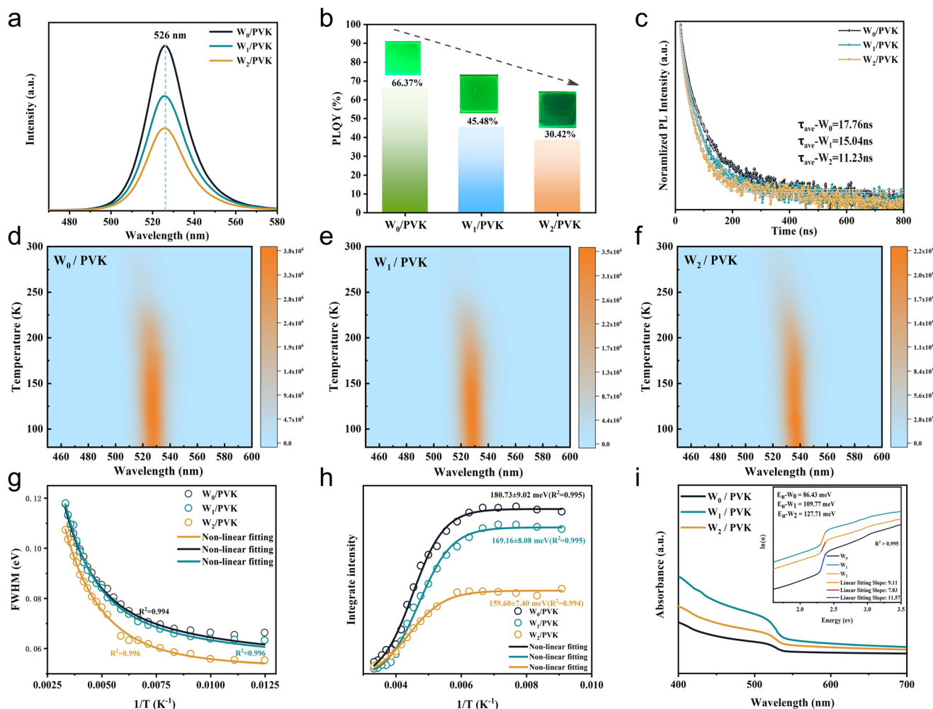
Fig. 2 Photophysical properties of the perovskite films on W_0/W_1/W_2 films. (a) PL spectra, (b) PLQY spectra, (c) TRPL spectra, (d, e and f) temperature-dependent PL spectra of the perovskite films on W_0/W_1/W_2 , (g) FWHM, (h) integrated PL intensity as a function of reciprocal temperature, (i) UV-vis and Urbach energy spectra of the perovskite films on W_0/W_1/W_2 films.
