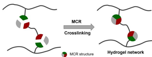
Fig. 1 The role of MCRs as crosslinking reactions.
