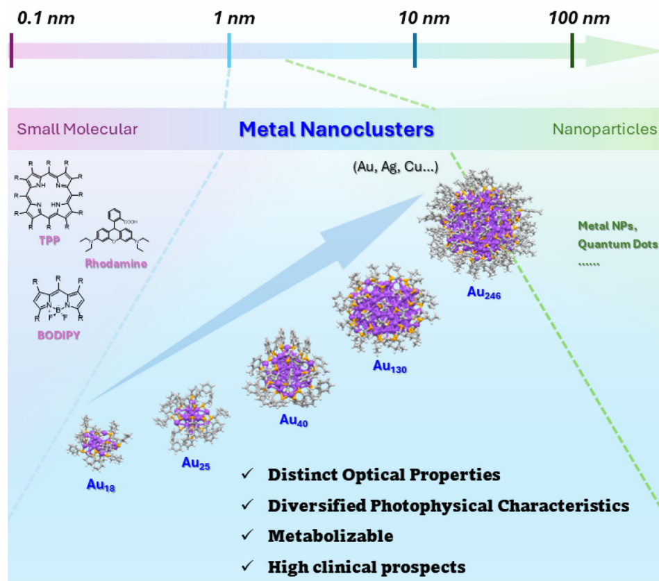
Scheme 1 Three kinds of optical probe materials with size increased.
