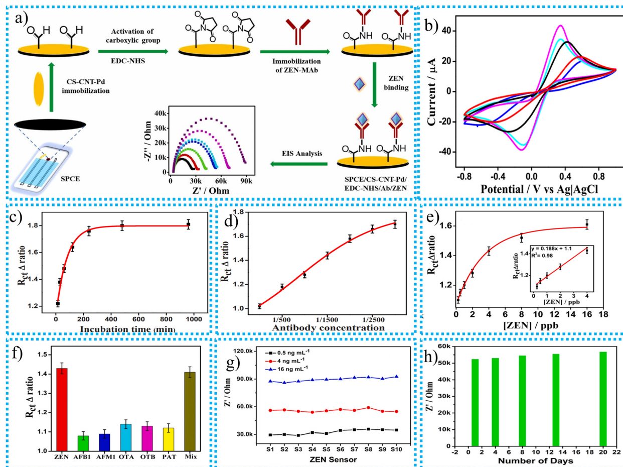
Fig. 12 (a) The CNT-based CSCNT-Pd-based immunosensor synthesis procedure, (b) CV curves for the impact of modification on the SPCE electrode, (c) electrochemical impedimetric responses ( \Delta_{\text{ratio}} ) of the SPCE/CS-CNT-Pd/ZEN-MAb modified electrode after incubation with 4 \text{ ng mL}^{-1} of ZEN at different incubation time intervals, (d) impedimetric responses of the SPCE/CS-CNT-Pd/ZEN-MAb modified electrode to varying concentrations of antibody (ZEN-MAb), (e) the calibration curve of the ZEN immunosensor based on the change in R_{\text{ct}} , (f) electrochemical impedimetric responses of the fabricated immunosensor, (g) impedance responses of ten independent immunosensor sets towards ZEN detection, (h) impedance responses of the ZEN immunosensor for 20 days under ambient conditions toward the detection of 2.0 \text{ ng mL}^{-1} of ZEN. 174
