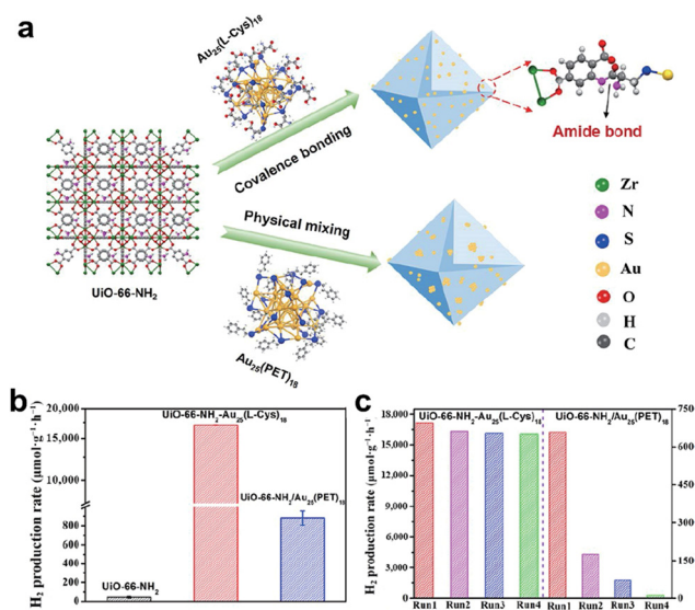
Fig. 12 (a) Schematic diagram of Au 25 (L-Cys) 18 bound to UiO-66-NH 2 through covalent bridge strategy. (b) Comparison of the photocatalytic H 2 production performance of UiO-66-NH 2 , covalent bonded UiO-66-NH 2 -Au 25 (L-Cys) 18 and physically mixed UiO-66-NH 2 /Au 25 (PET) 18 with ErB and TEOA as the photosensitizer and sacrificial agent. The light source was a 300 W xenon lamp with a >420 nm filter. (c) Comparison of cycling stability of UiO-66-NH 2 -Au 25 (L-Cys) 18 and UiO-66-NH 2 /Au 25 (PET) 18 . Reproduced with permission from ref. 82. Copyright 2023 Springer Nature.
