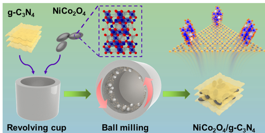
Fig. 1 Schematic illustration of the preparation of NiCo 2 O 4 /g-C 3 N 4 composites.
