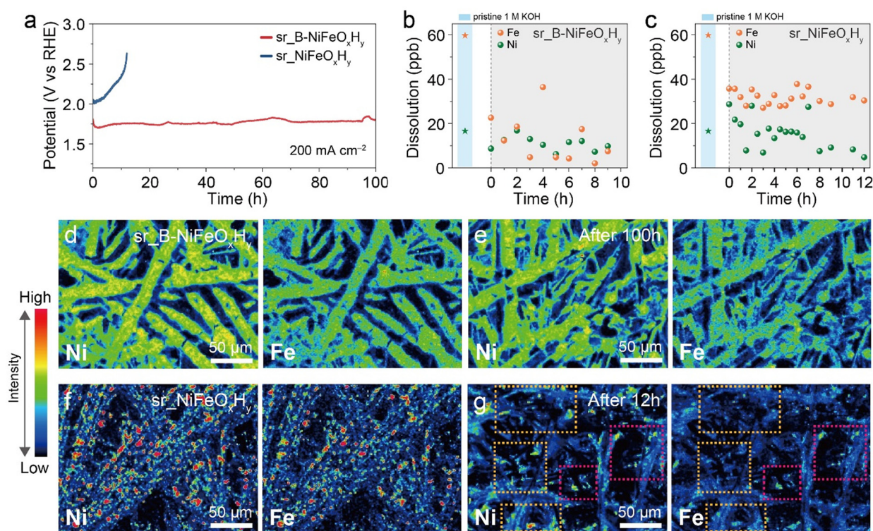
Fig. 4 (a) Long-term stability test of \text{sr}_\text{B-NiFeO}_x\text{H}_y and \text{sr}_\text{NiFeO}_x\text{H}_y at a current density of 200 \text{ mA cm}^{-2} and the corresponding inductively coupled plasma-mass spectrometry (ICP-MS) trace (b) \text{sr}_\text{B-NiFeO}_x\text{H}_y and (c) \text{sr}_\text{NiFeO}_x\text{H}_y during the long-term stability test. Electron probe microanalysis (EPMA) of (d and e) \text{sr}_\text{B-NiFeO}_x\text{H}_y and (f and g) \text{sr}_\text{NiFeO}_x\text{H}_y for Ni and Fe after 10 and 12 hours at a current density of 200 \text{ mA cm}^{-2} , respectively. The highlighted areas indicate areas with similar Ni intensities. Orange and red boxes indicate Fe-poor regions and regions where Fe remained relatively intact, respectively.
