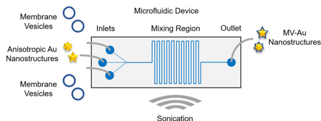
Fig. 1 Schematic of the microfluidic device used for the synthesis of the cell membrane vesicle-encapsulated anisotropic Au nanostructures. The device consists of three inlet ports and an outlet port connected by a serpentine-shaped mixing region. It was immersed in a bath sonicator throughout the nanostructure synthesis process.
