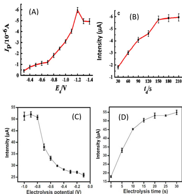
Fig. 9 Electrolysis potential (A) and electrolysis time (B) in 10 \mu M Pb^{2+} in 0.1 M acetate buffer (pH 5.4) recorded at a \beta -CD-rGO/GCE. This figure has been reproduced from ref. 51 with permission from Springer, copyright 2016. Electrolysis potential (C) and electrolysis time (D) in 2 \mu M Pb^{2+} in 0.1 M acetate buffer (pH 5) recorded at a GCE/NHAPPO.5-CA- \beta -CD. This figure has been reproduced from ref. 40 with permission from Springer-Verlag GmbH Germany., copyright 2021.
