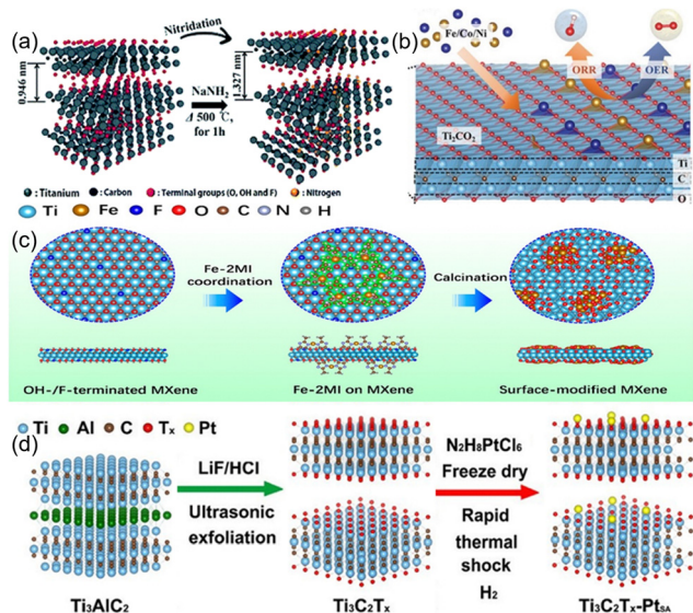
Fig. 4 (a) Synthesis procedures for the N- \text{Ti}_2\text{CT}_x nanosheets and their dispersion. 46 Copyright 2018, Royal Society of Chemistry. (b) Mechanisms for the formation of Fe/Co/Ni-DACs based on \text{Ti}_2\text{CO}_2 and for the electrocatalytic reactions in aqueous electrolytes. 52 Copyright 2021, Wiley. (c) Schematic illustration for the preparation procedure of the surface-tuned MXene/ \text{TiFeO}_x nanosheets. 51 Copyright 2020, American Chemical Society. (d) Schematic illustration of constructing Pt single atoms on monolayer \text{Ti}_3\text{C}_2\text{T}_x . 53 Copyright 2022, American Chemical Society.
