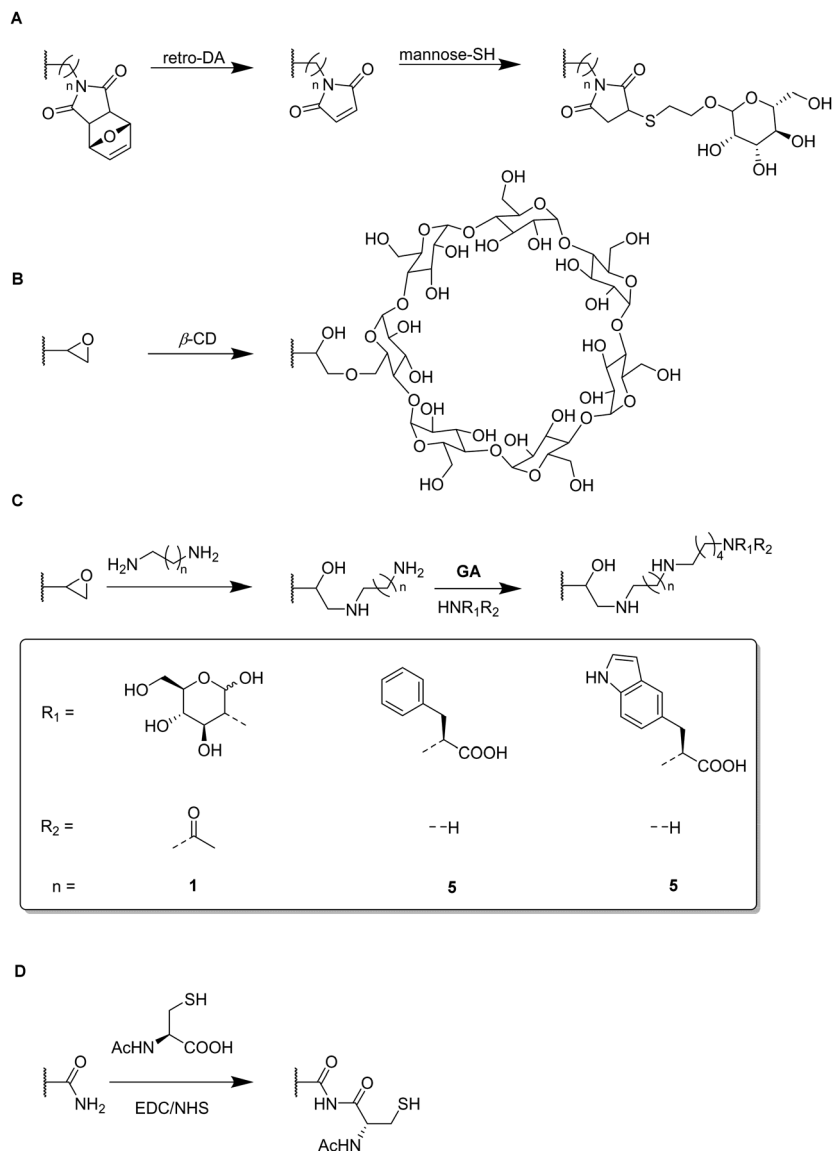
Fig. 18 Schematic representation of various strategies for the functionalization of synthetic polymer based cryogels with sugars and amino acids. Thiol-maleimide click reaction for the introduction of mannose-thiol after retro-Diels Alder (retro-DA) reaction (A). Direct coupling of nucleophiles such as cyclodextrin (CD) to epoxide cryogel surfaces (B), coupling of nucleophiles using the glutaraldehyde method via spacer formation (C) and EDC/NHS coupling (D).
