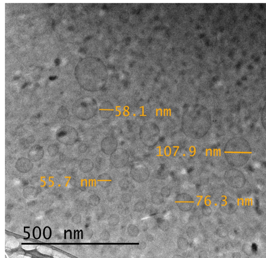
Fig. 5 Cryo-TEM image of the polymersomes with diblock copolymer: motor ratios of 100:2.
