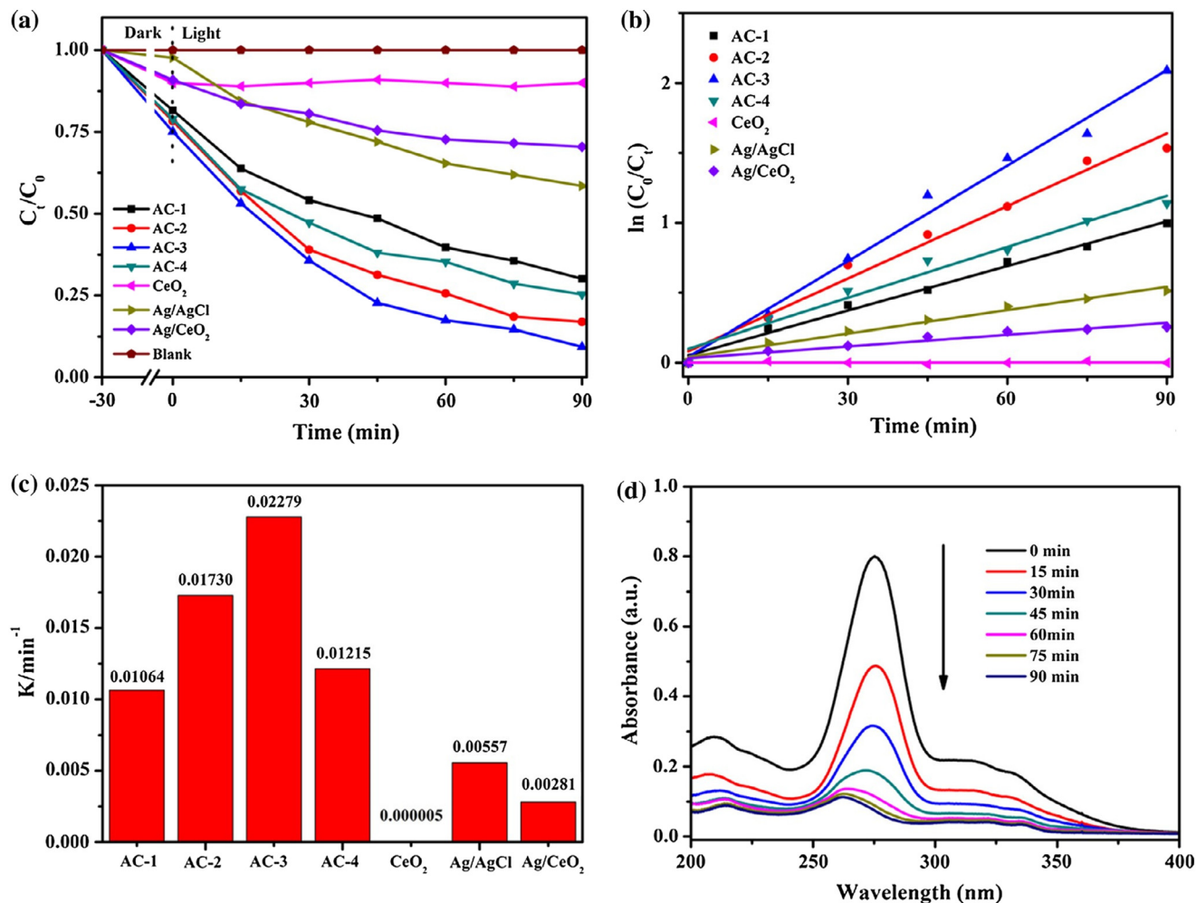
Fig. 14 (a) Photocatalytic degradation of NOF curves; (b) kinetic curves of NOF degradation; (c) apparent rate constants for the degradation of NOF; (d) time-dependent UV-vis spectra of NOF solution for AC-3 sample (Ag/AgCl-CeO 2 ). Reproduced from ref. 383 with permission from Elsevier (2017).
