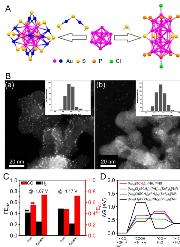
Fig. 20 (A) Atom packing structures of Au 25 nanosphere ( [Au_{25}(PET)_{18}]^- ) and nanorod ( [Au_{25}(PPh_3)_{10}(PET)_5Cl_2]^{2+} ). (B) STEM images and particle size histograms of (a) Au 25 nanosphere and (b) nanorod supported on carbon black. (C) FE_{CO} and FE_{H_2} at the potential of -1.07 and -1.17 V over Au 25 nanosphere and nanorod, respectively. (D) Free energy diagrams ( \Delta G ) for CO 2 reduction to CO on the ligand-removed NCs at 0 V vs. RHE. The black, blue, green, and red lines represent CO 2 reduction to CO on the nanorod with PH 3 removed, the nanorod with -SCH 3 removed, the nanorod with -Cl removed, and on the nanosphere with -SCH 3 removed, respectively. Panels (A)–(D) are reproduced with permission from ref. 299. Copyright 2018 American Chemical Society.
