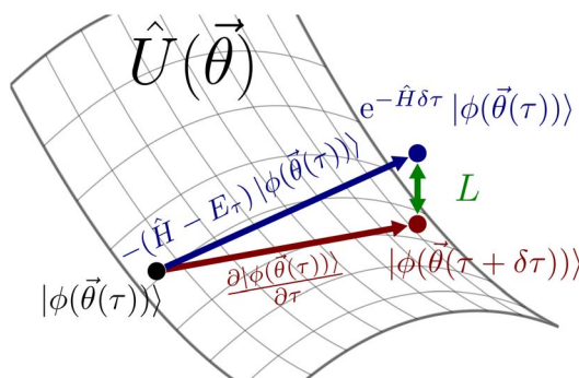
Fig. 2 VarQITE is an approximation to QITE. The McLachlan distance, L (green) quantifies how far a point on the manifold given by the ansatz \hat{U}(\vec{\theta}) (red) is from the ideal QITE path (blue). VarQITE minimizes this distance after each small imaginary time step \delta\tau .
