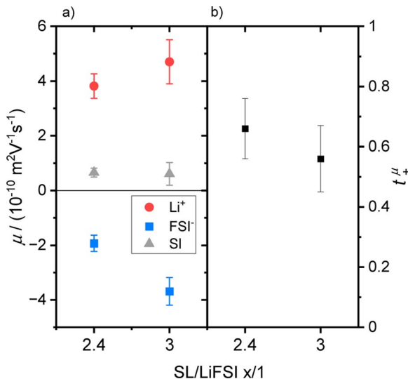
Fig. 3 (a) Mobility data of SL/LiFSI = x/1 with x = 2.4 and 3 for \text{Li}^+ (red dots), \text{FSI}^- (blue squares) and \text{SL} (grey triangles) and (b) the resulting \text{Li}^+ transference numbers t_+^\mu .
