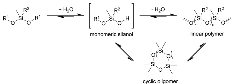
Scheme 1 Condensation of siloxanes. Reaction conditions: TF-Sil \alpha -Strep (cat.), toluene, 70 °C. \text{R}^1 = Me or (4-methoxy)phenyl; \text{R}^2 = Me or Ph; n = 1–3.
