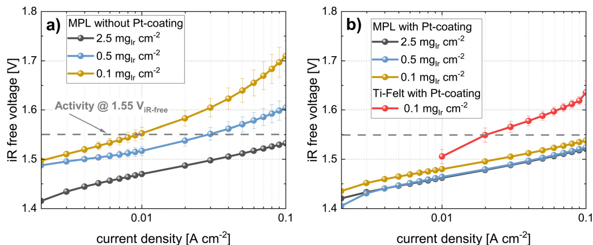
Fig. 9 Semi-logarithmic plots of the iR -free cell voltage vs. current density (Tafel-plots) for all loadings in CCM configuration (a) MPLs without Pt-coating (b) MPLs with Pt-coating and comparison with Ti-felt reference with Pt-coating; all measurements with N115, at T = 80^\circ\text{C} and 10 bar balanced pressure.
