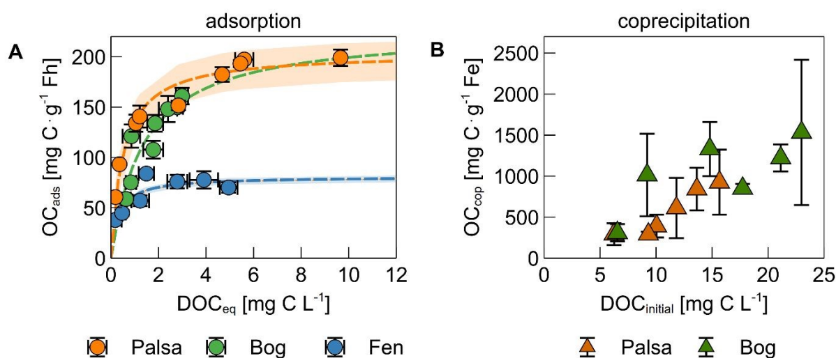
Figure 1. (A) Adsorption isotherm of water-extractable organic matter (WEOM) from different permafrost thaw stages on ferrihydrite (Fh). The mass of OC adsorbed ( \text{mg C g}^{-1} \text{Fh} ) is displayed against the equilibrium DOC concentration in solution after sorption. Data are denoted by circles and the Langmuir fit and 95% confidence interval is displayed as a dashed line and shaded area, respectively. The sorption experiments were performed at pH 4.5 for palsa, pH 4.5 for bog, and pH 6.0 for fen WEOM to represent environmentally relevant conditions. (B) Quantity of coprecipitated organic carbon ( \text{mg C g}^{-1} \text{Fe} ) as a function of the initial DOC (triangles). All data points and error bars represent the average and standard deviation of experimental triplicates. Note that the units and range of the y-axis are different for the two graphs.
