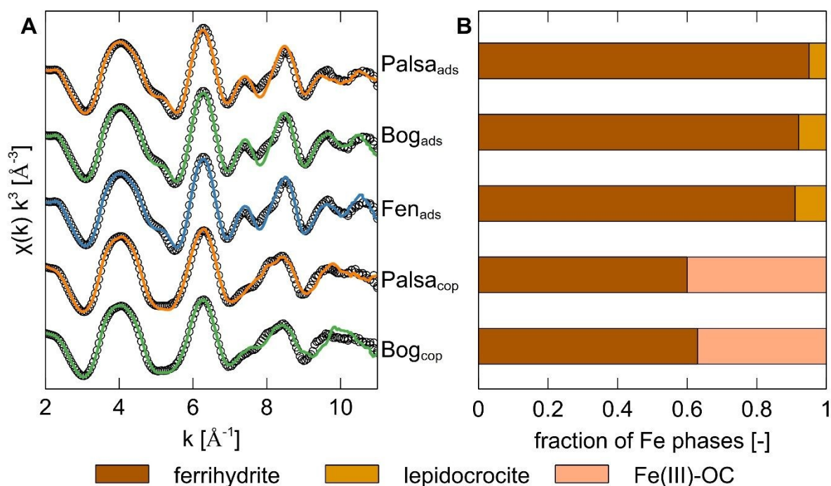
Figure 2. (A) Iron K -edge k^3 -weighted EXAFS spectra and linear combination fits (2 to 11 \text{\AA}^{-1} ) of ferrihydrite with adsorbed WEOM (ads) from palsa, bog and fen, and Fe-OC coprecipitates (cop) synthesized with WEOM from palsa and bog. Experimental data is displayed as coloured lines and linear combination fits as black circles (see fit parameters in Table S6). (B) Bar plot showing relative abundances of different Fe phases in the post-adsorption and post-coprecipitation mineral phases. The same labelling as for graph (A) applies here. Fe(III)-OC was fit using Fe(III)-citrate as a reference.
