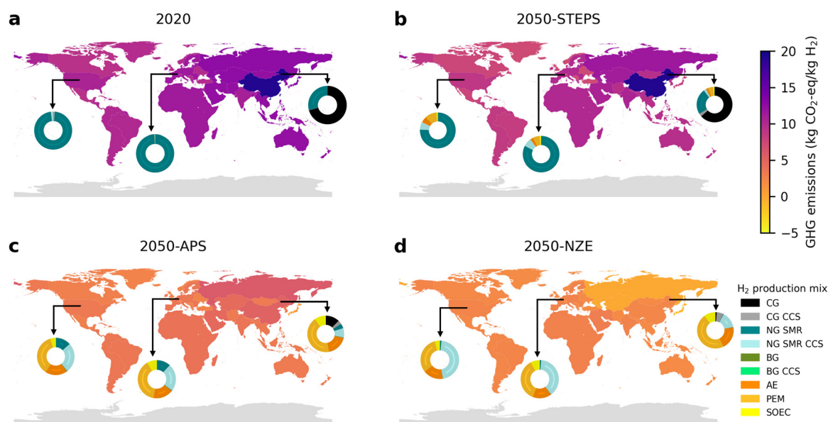
Fig. 5 GHG emissions of one kg H 2 of regional markets in 2020 and 2050. (a) Shows GHG emissions of per kg H 2 from 15 regional H 2 market, as well as market share of different H 2 technologies in China, the USA and the EU in 2020. (b)–(d) show these values in 2050 in three scenarios. In the legend of H 2 production mix, CG = coal gasification, NG SMR = steam methane reforming of natural, BG = biomass gasification, CCS = carbon capture and storage, AE = alkaline electrolyzer, PEM = proton exchange membrane electrolyzer and SOEC = solid oxide electrolysis cell. There is no data for the Antarctic.
