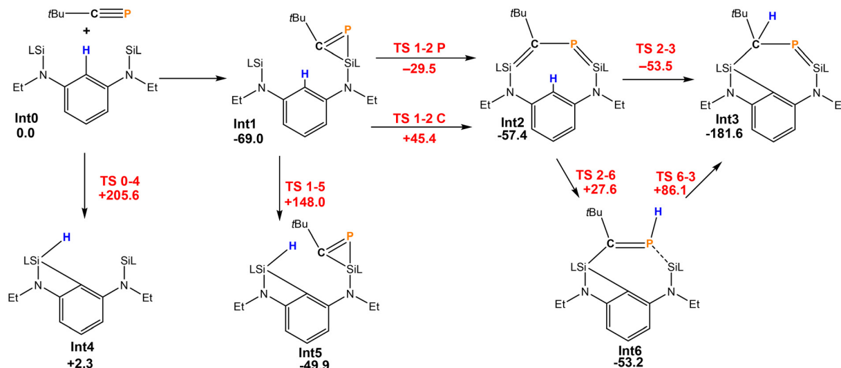
Scheme 3 Reaction of [LSiCSiL] and t BuC≡P (energies in \text{kJ mol}^{-1} , intermediates in black, transition states in red).
