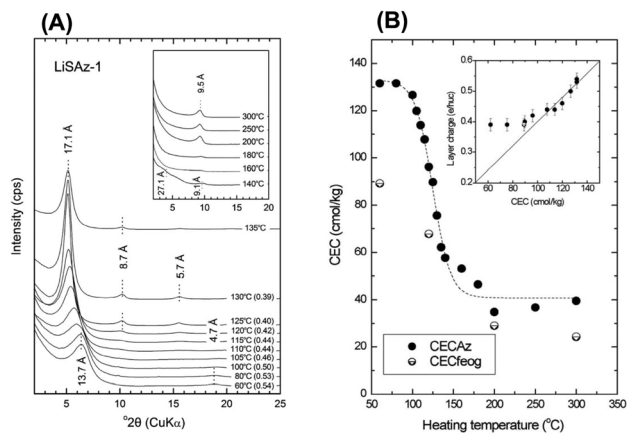
Fig. 24 (A) Room-temperature XRD patterns of K-saturated and ethylene glycol-solvated LISAz-1 samples pre-heated in the range of 60–135 °C for 24 h. Layer charges (e - /Si, Al 4 O 10 (OH) 2 ) calculated according to ref. 465 are shown in parentheses. The inset shows the patterns of the corresponding samples heated at higher temperatures and up to 300 °C. Note the appearance of a new peak ~9.5 Å, which indicates collapsed layers. (B) Dependence of CEC on the heating temperature. The inset compares the layer charge and CEC data of the same samples. Reprinted with permission from ref. 466. Copyright 2013, Springer.
