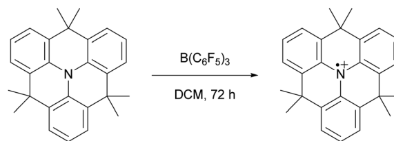
Scheme 2 The first reported example of an SET between B(C_6F_5)_3 and an organic electron donor, in this case a triarylamine, as reported by Wang et al.
