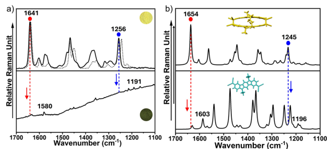
Fig. 13 (a) Top: FT-Raman spectra at \lambda_{\text{exc}} = 1064 nm of the yellow powder of (m-ICz-CN) 2 (black line) and its brominated precursor m-ICz-Br (black dots). Bottom: Raman spectrum at \lambda_{\text{exc}} = 785 nm of isolated diradical m-ICz-CN in the solid state at 410 K. (b) Theoretical Raman spectra of (m-ICz-CN) 2 (top) and m-ICz-CN (down) at the M06-2X/6-31G** level.
