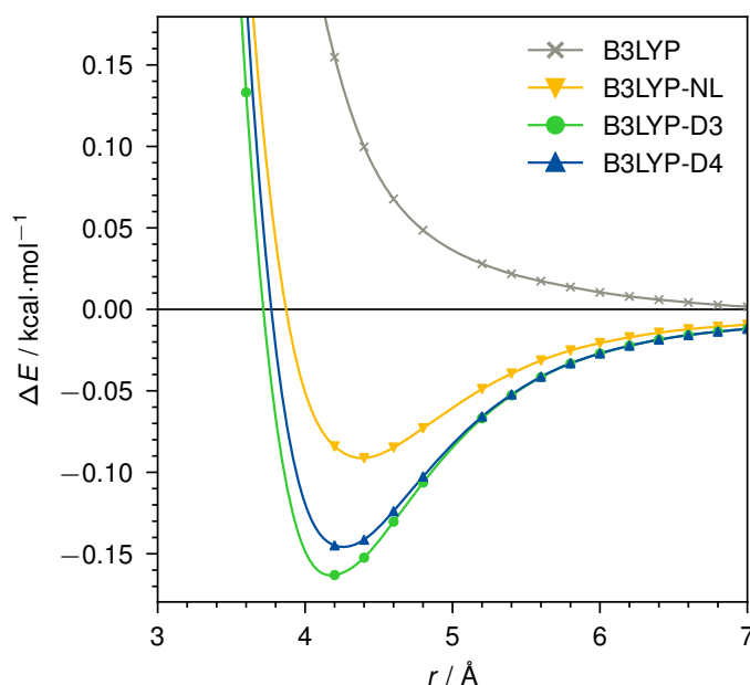
Fig. 5 Dissociation curve of \text{No}\text{---Ne} for B3LYP/def2-TZVP without dispersion correction, with NL, D3, or D4.
