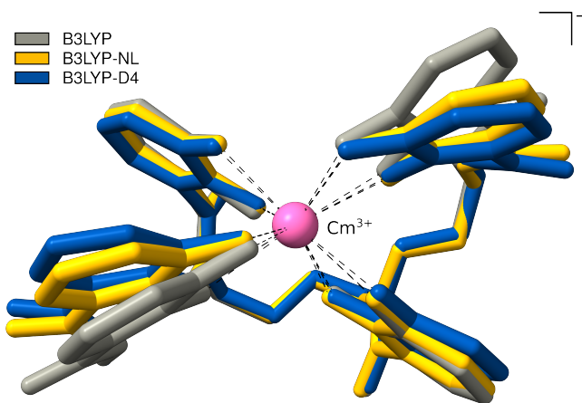
Fig. 7 PBE0-D4/def2-SVP Optimized structures of \text{Cm}^{3+}\text{-4OL} with B3LYP, B3LYP-NL, and B3LYP-D4. Hydrogen atoms are omitted for clarity.
