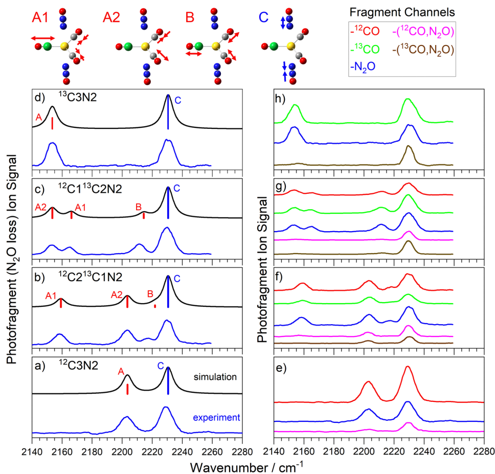
Fig. 4 (a)–(d) Comparison of experimental and simulated infrared action spectra of Au(^{13/12}CO)_3(N_2O)_2^+ complexes, recorded in the N_2O loss channel. (e)–(h) Spectra recorded in different dissociation product channels, colour coded as above.
