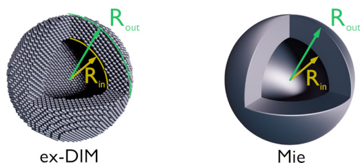
Fig. 8 Representations of R_{\text{out}} and R_{\text{in}} for Ex-DIM and Mie models of nano-shells. The Ex-DIM radius of the atoms corresponds to the effective radius. From ref. 143.
