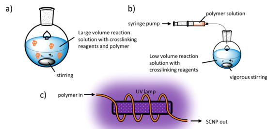
Fig. 4 Illustration of experimental procedures for the synthesis of SCNPs using (a) a large volume reaction solution with a low concentration of polymer, (b) the continuous-addition protocol, and (c) a photochemical flow reactor.
