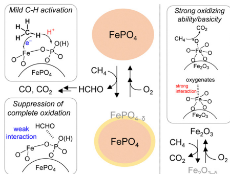
Fig. 13 Proposed reaction mechanism for oxidation of \text{CH}_4 over \text{FePO}_4 into HCHO with \text{O}_2 using \text{FePO}_4 and complete oxidation of \text{CH}_4 over \text{Fe}_2\text{O}_3 into \text{CO}_2 with \text{O}_2 using \text{Fe}_2\text{O}_3 . (Reproduced from ref. 53 with permission from Royal Society of Chemistry).
