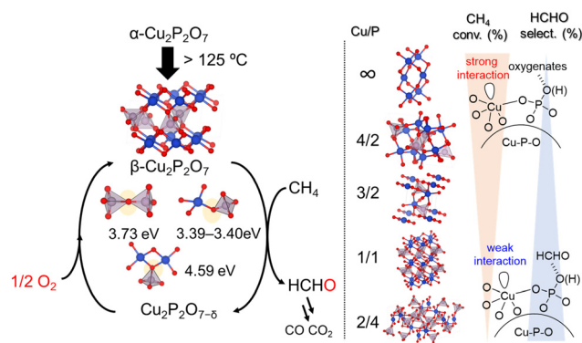
Fig. 15 Proposed reaction mechanism for oxidation of \text{CH}_4 over copper phosphates into HCHO with \text{O}_2 . (Reproduced from ref. 51 with permission from The American Chemical Society).
