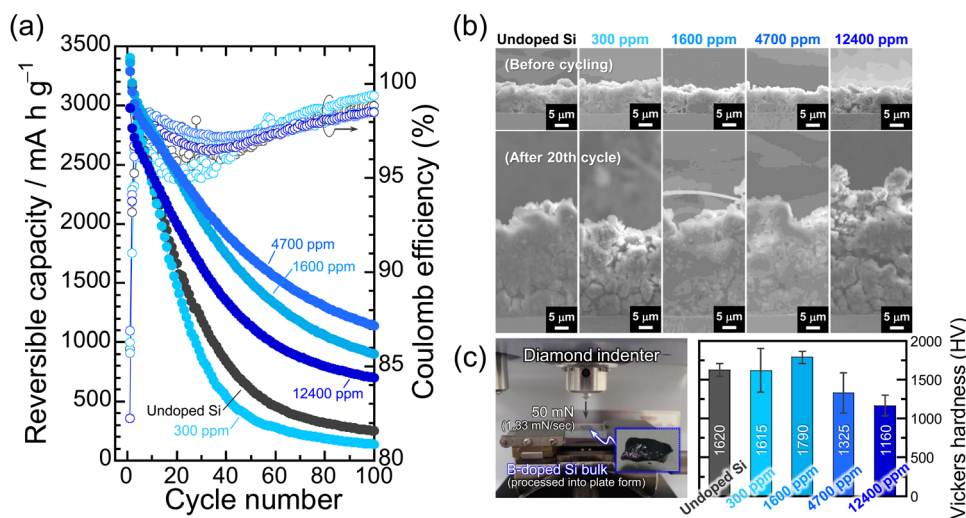
Fig. 3 (a) Dependence of the discharge capacities and Coulomb efficiencies on cycle number for undoped-Si and B-doped Si electrodes (300, 1600, 4700, and 12 400 ppm) at 0.1C. (b) Cross-sectional SEM images of the electrodes before and after the 20th cycle. (c) Vickers hardness of the Si bulk samples. The Vickers hardness was measured using a diamond indenter with a fixed force (load: 50 mN).
