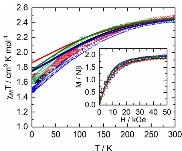
Fig. 1 Thermal dependence of \chi_{\text{M}}T for (a) [( S )-1] n (black squares), (b) [( S,S,S )-2] n (blue circles), (c) [( S )-3] n (red up-triangles) and (d) [( S,S,S )-4] n (green down-triangles). Inset: Field variation of the magnetization measured at 2 K for [( S )-1] n (black squares), (b) [( S,S,S )-2] n (blue circles), (c) [( S )-3] n (red up-triangles) and (d) [( S,S,S )-4] n (green down-triangles). Full lines correspond to the ab initio computational results (see text for details).
