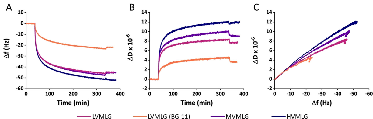
Fig. 3 Adsorption of MLGs on TCNF. Changes is (A) frequency, (B) dissipation factor, and (C) dissipation factor as a function of frequency during adsorption of 0.01 wt% MLG solutions on TCNF surfaces. A baseline for TCNF surfaces was first obtained, after which MLG solutions were introduced at around 30 min. Lastly, a rinsing step was applied at 350 min. Adsorption of LVMLG in both water and BG-11 growth medium is shown. 15 MHz, f_0 = 5 MHz, n = 3 .
