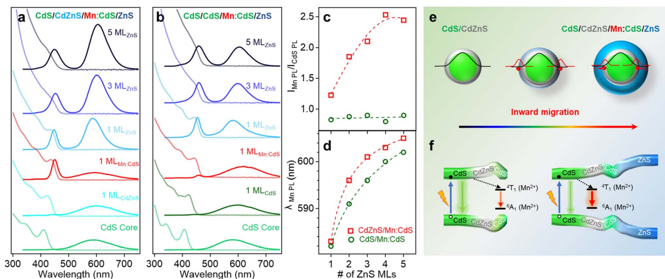
Fig. 5 (a and b) Normalized absorption and PL spectra of (a) CdS/CdZnS/Mn:CdS/ZnS (1–5 ML S ) and (b) CdS/CdS/Mn:CdS/ZnS (1–5 ML S ) core/multi-shell QDs. (c) The PL Intensity ratio of Mn(II) and CdS host lattice and (d) the changes of Mn(II) PL peak position as a function of ZnS shell thickness. (e) Schematic of the dopant inward migration by inserted CdZnS alloyed trap layer and (f) the band alignment of the CdS/CdZnS/Mn:CdS/ZnS core/multi-shell QDs.
