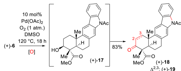
Scheme 4 Synthesis of a pentacyclic framework under oxidative C–N bond formation.
