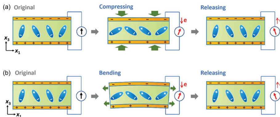
Fig. 4 Illustration of working mechanism of a piezoelectric sensor when (a) mechanical pressure or (b) strain is applied to the device. Reproduced with permission from ref. 101 Copyright 2022 John Wiley and Sons.
