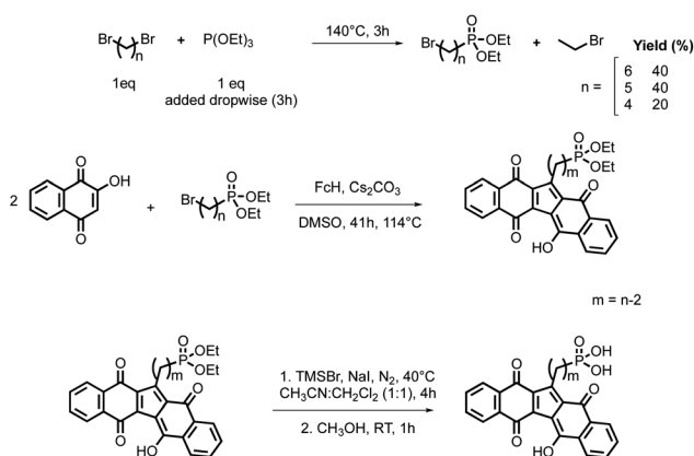
Scheme 3 Stepwise synthesis of KuQXPO 3 Et 2 (X = 2, 3, 4).
