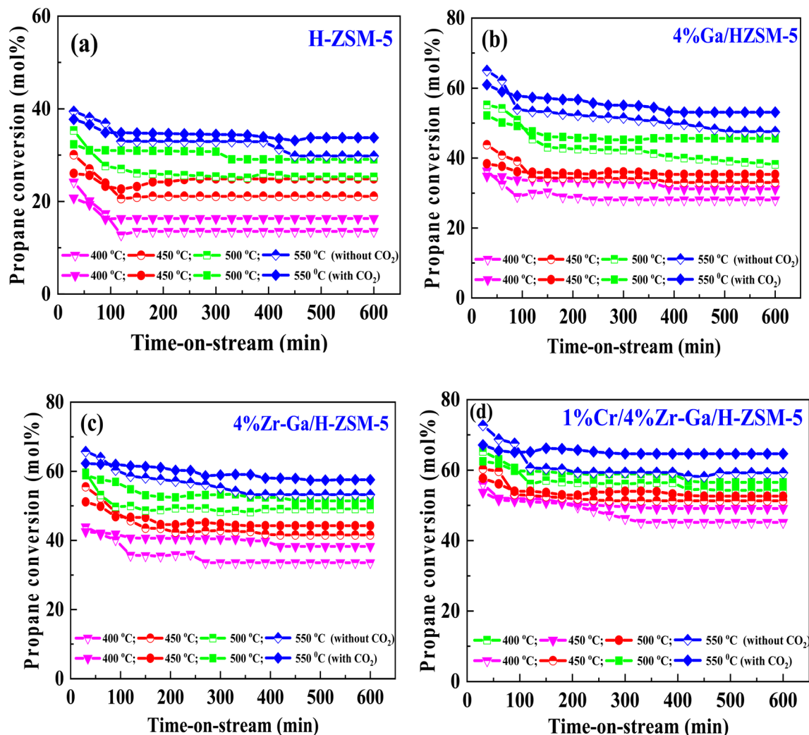
Fig. 6 Catalytic performance of (a) H-ZSM-5; (b) 4% Ga/H-ZSM-5; (c) 4% Zr-Ga/H-ZSM-5; and (d) 1% Cr/4% Zr-Ga/H-ZSM-5 catalysts. Reaction conditions: pressure, 1 bar; feed gas, C 3 H 8 /N 2 = 2.5/97.5 and C 3 H 8 /CO 2 /N 2 = 2.5/5/92.5; flow rate, 75 mL min -1 , WHSV, 4 Kg cat s -1 .
