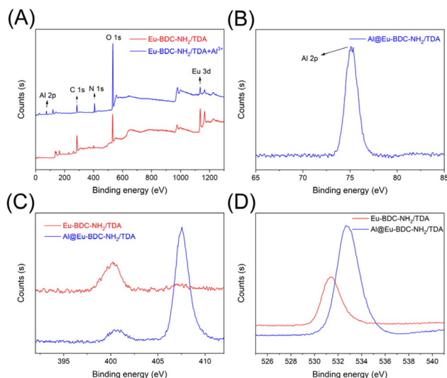
Fig. 7 (A) XPS spectra for Eu-BDC-NH 2 /TDA and Al@Eu-BDC-NH 2 /TDA. (B) XPS spectra for Al 2p in Al@Eu-BDC-NH 2 /TDA. (C) XPS spectra for N 1s in Eu-BDC-NH 2 /TDA and Al@Eu-BDC-NH 2 /TDA. (D) XPS spectra for O 1s in Eu-BDC-NH 2 /TDA and Al@Eu-BDC-NH 2 /TDA.
