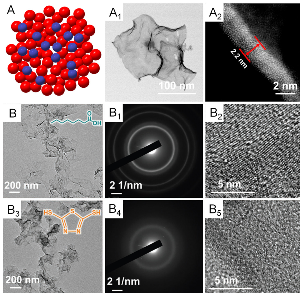
Fig. 9 Amorphization of metallenes. (A) Schematic illustration showing the atomic model of amorphous metallene with a disordered surface atomic arrangement. (A 1 ) TEM image and (A 2 ) the lateral HAADF-STEM image of amorphous Pd metallene doped with S atoms. Reproduced from ref. 72 with permission from American Chemical Society. Copyright 2022. (B) TEM image, (B 1 ) SAED pattern, and (B 2 ) HRTEM image of crystalline Pd metallene (the inset shows the molecular structure of octanoic acid). (B 3 ) TEM image, (B 4 ) SAED pattern, and (B 5 ) HRTEM image of amorphous Pd metallene. (The inset shows the molecular structure of bismuthiol I). Reproduced from ref. 75 with permission from Wiley-VCH. Copyright 2020.
