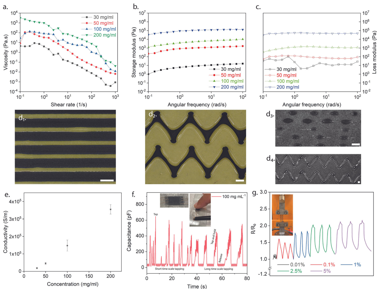
Fig. 4 Demonstrative characterizations of Ti 3 C 2 T x inks. (a) Flow sweep test showing the change in viscosity of the ink concentrations with increasing shear rate. (b) and (c) Oscillation frequency test showing variations of storage moduli ( G' and G'' , respectively) against angular frequency. (d 1 )–(d 4 ) Different patterns of MXene printed using the DIW method (d 1 ) Scale 500 μm; (d 2–3 ) Scale 1000 μm. (e) Conductivity vs. concentration plot of aqueous ink solutions. (f) An interdigitated capacitor with parallel printed lines of MXene displaying capacitive sensing responding to index finger. (g) Strain sensing performance at strain loading from 0.01–5%.
