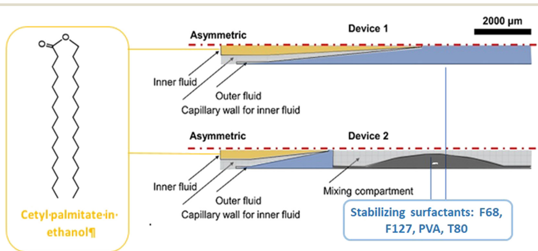
Fig. 8 Schematic representation of microfluidic devices 1 and 2. As for device 1, the outflow is collected and cooled; for device 2, the outflow is further connected to a three-port valve with continuous air pumping (mixing compartment). Image adapted from ref. 120.
