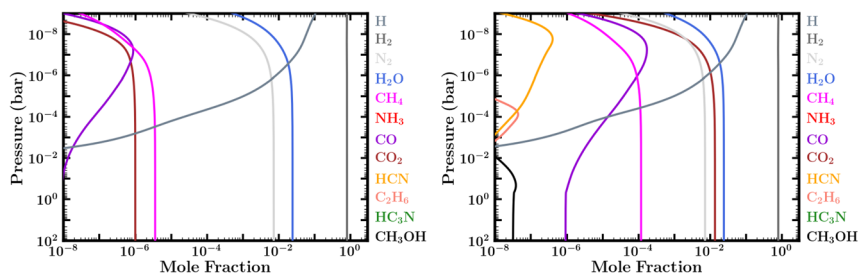
Fig. 4 Steady-state mixing-ratio profiles considering an atmosphere with lower boundary conditions of an active ocean surface with prescribed N 2 , H 2 O, and CO 2 mixing ratios and assuming the PT1 temperature profile in Fig. 2. Left: Abundances assuming a low CO 2 mixing ratio of 10 −6 at the atmosphere–ocean boundary, corresponding to case 10 in Table 1. Right: Abundances assuming a high CO 2 mixing ratio of ~1.4 × 10 −2 at the atmosphere–ocean boundary, corresponding to Case 9 in Table 1.
