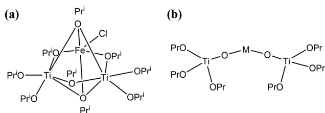
Fig. 22 Molecular structures of (a) [\text{FeCl}\{\text{Ti}_2(\text{OPr}^i)_9\}] , (b) [\text{M}\{\text{O-Ti}(\text{OPr}^i)_3\}_2] ( \text{M} = \text{Mg}, \text{Mn}, \text{Fe}, \text{Co}, \text{Zn}, \text{Sn} ).
