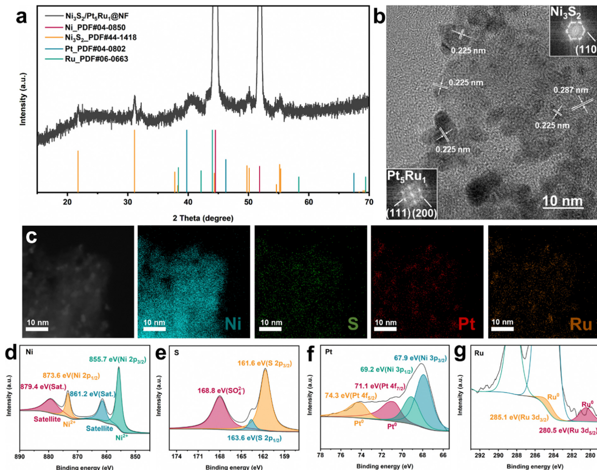
Fig. 1 Structural and microstructure characterizations of Ni 3 S 2 /Pt 5 Ru 1 @NF. (a) XRD pattern, (b) HRTEM image and the corresponding FFT patterns, (c) STEM image and the corresponding EDX elemental mapping images, and XPS spectra of (d) Ni 2p, (e) S 2p, (f) Pt 4f, and (g) Ru 3d.
