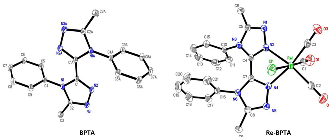
Fig. 2 Molecular views of ligand BPTA and complex Re-BPTA. Hydrogen atoms are not represented for the sake of clarity. Displacement ellipsoids are drawn at 30% probability.
