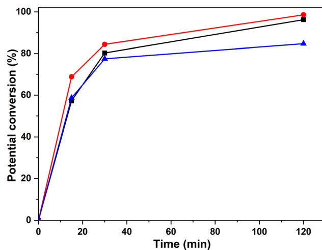
Fig. 9 Potential percentage of inter-unit bond conversion corresponding to the bonds \beta -O-4( \beta ) (–■–), \beta -O-4'( \alpha ) (–●–) and \beta -5' (–▲–), obtained by ^1\text{H} -NMR spectra with the integration of the areas at \delta_{\text{H}} of 4.19 ppm, 4.98 ppm and 5.08 ppm, respectively.
